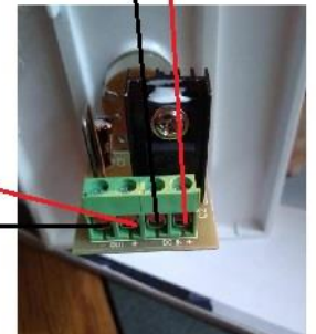
single channel dimmer shown here for illustration purposes - check output wiring of your specific dimmer
