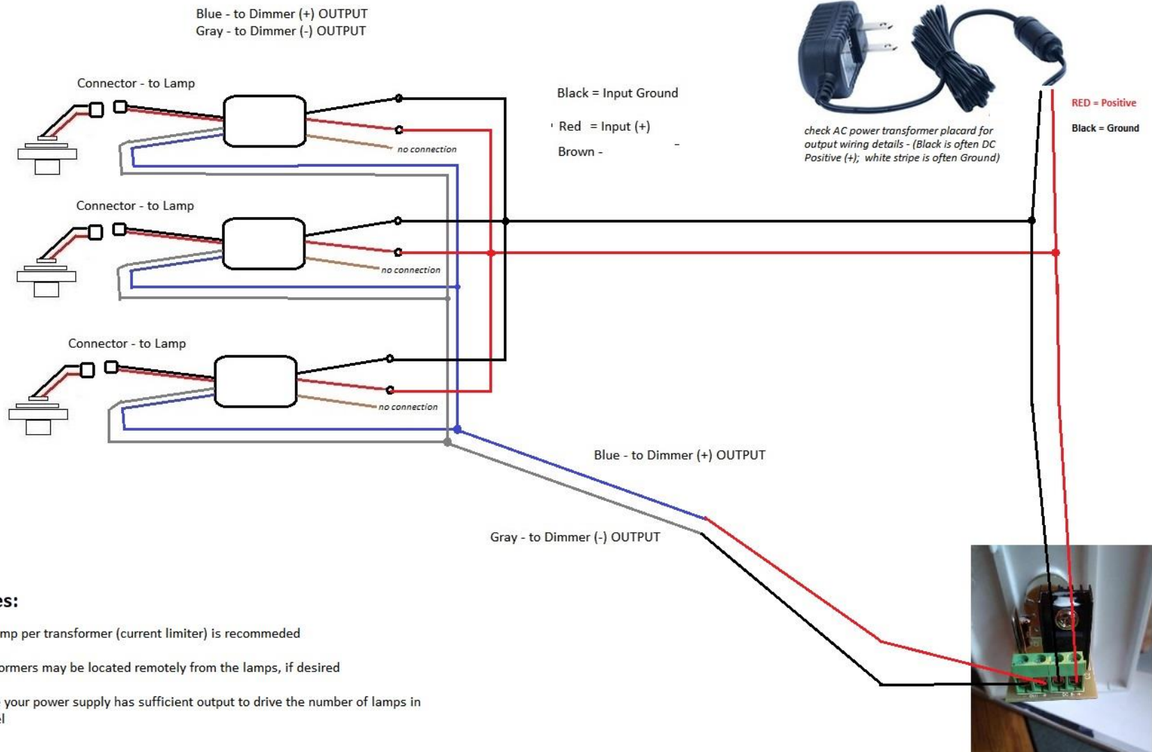
single channel dimmer shown here for illustration purposes - check output wiring of your specific dimmer
